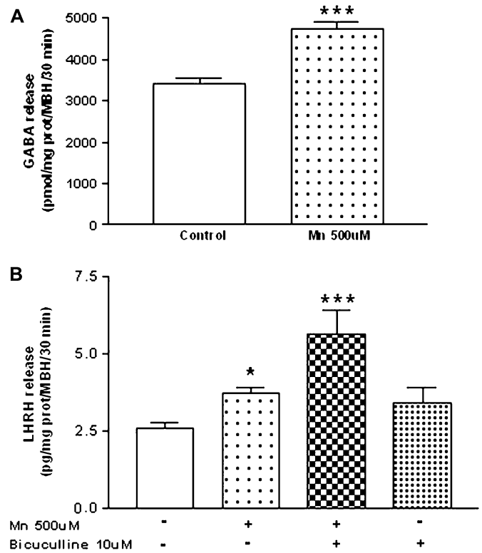
FIG. 7. Effect of \text{MnCl}_2 on GABA release (A) and the action of bicuculline (B), a \text{GABA}_A receptor antagonist, on \text{MnCl}_2 -stimulated LHRH release from MBH in vitro . Note that both GABA and LHRH release were increased by \text{MnCl}_2 , and that bicuculline enhanced \text{MnCl}_2 -induced LHRH secretion but had no effect when incubated alone. * p < 0.05 , and *** p < 0.001 versus control. Values represent mean \pm SEM. The - or + symbols indicate the absence or presence of \text{MnCl}_2 and bicuculline in the incubation medium.
