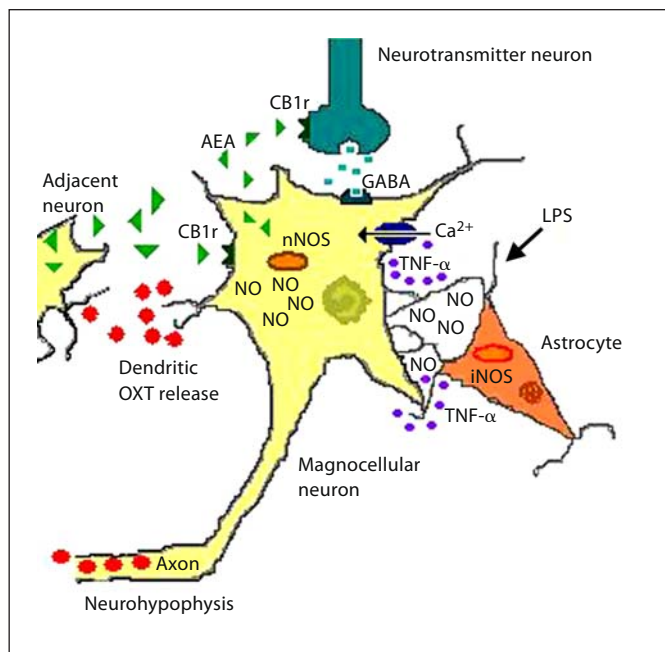
Fig. 1. Postulated mechanism for endocannabinoid participation in OXT release from PVN and SON hypothalamic nuclei after LPS challenge: LPS challenge increases the brain production of cytokines, between them TNF- \alpha . There is also iNOS activation from astrocytes with an increase in NO production. These factors and Ca 2+ depolarization induce the activation of magnocellular neurons increasing the release of OXT. Also, LPS increase the synthesis of AEA which stimulates nNOS activity, increasing NO stimulating OXT release. Furthermore, AEA acts as a retrograde messenger on CB 1 receptors present on presynaptic terminals of adjacent neurons. Since CB 1 are G i/o -coupled receptors, AEA inhibition of inhibitory GABA adds to the augmentation of OXT release.
